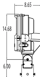
TM/TS - Tenon Mount Luminaire EPA of 1.89 Ft 2 and max weight 28 lbs.
